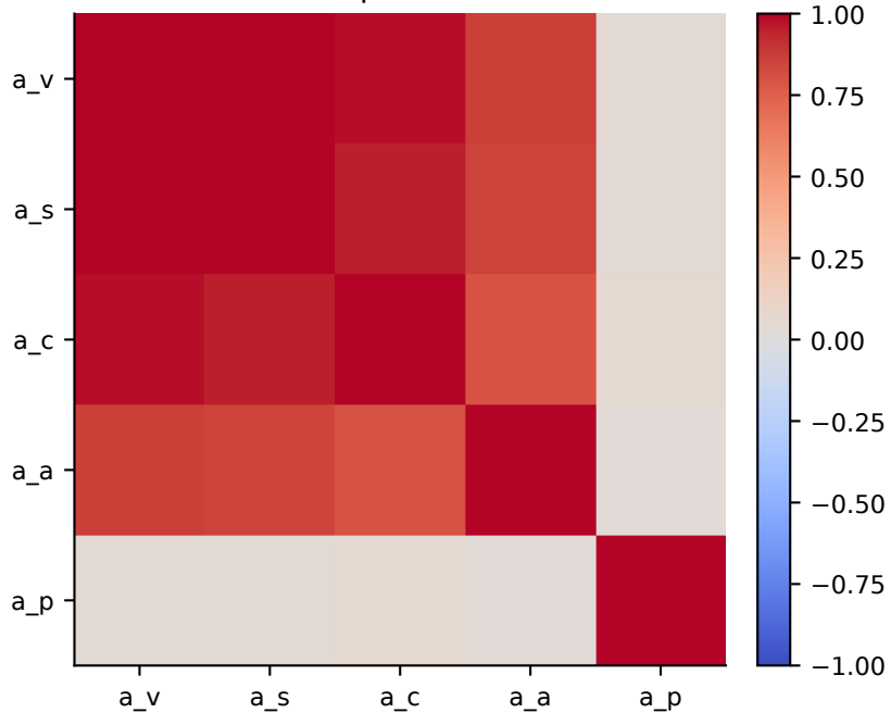
AME2020 bootstrap coefficient correlation
