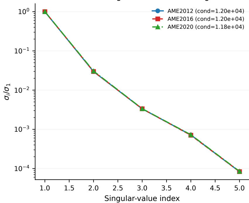
SEMF design-matrix conditioning
