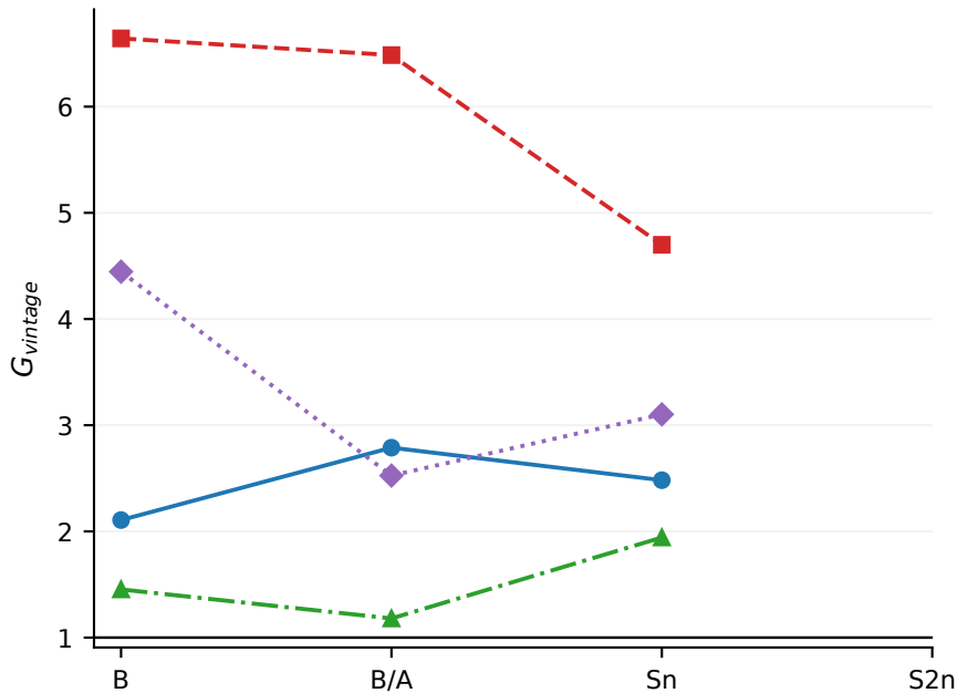
AME2012 -> AME2016 development
