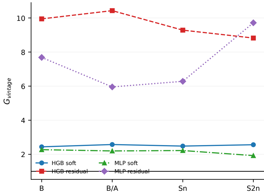
AME2016 -> AME2020 confirmation
