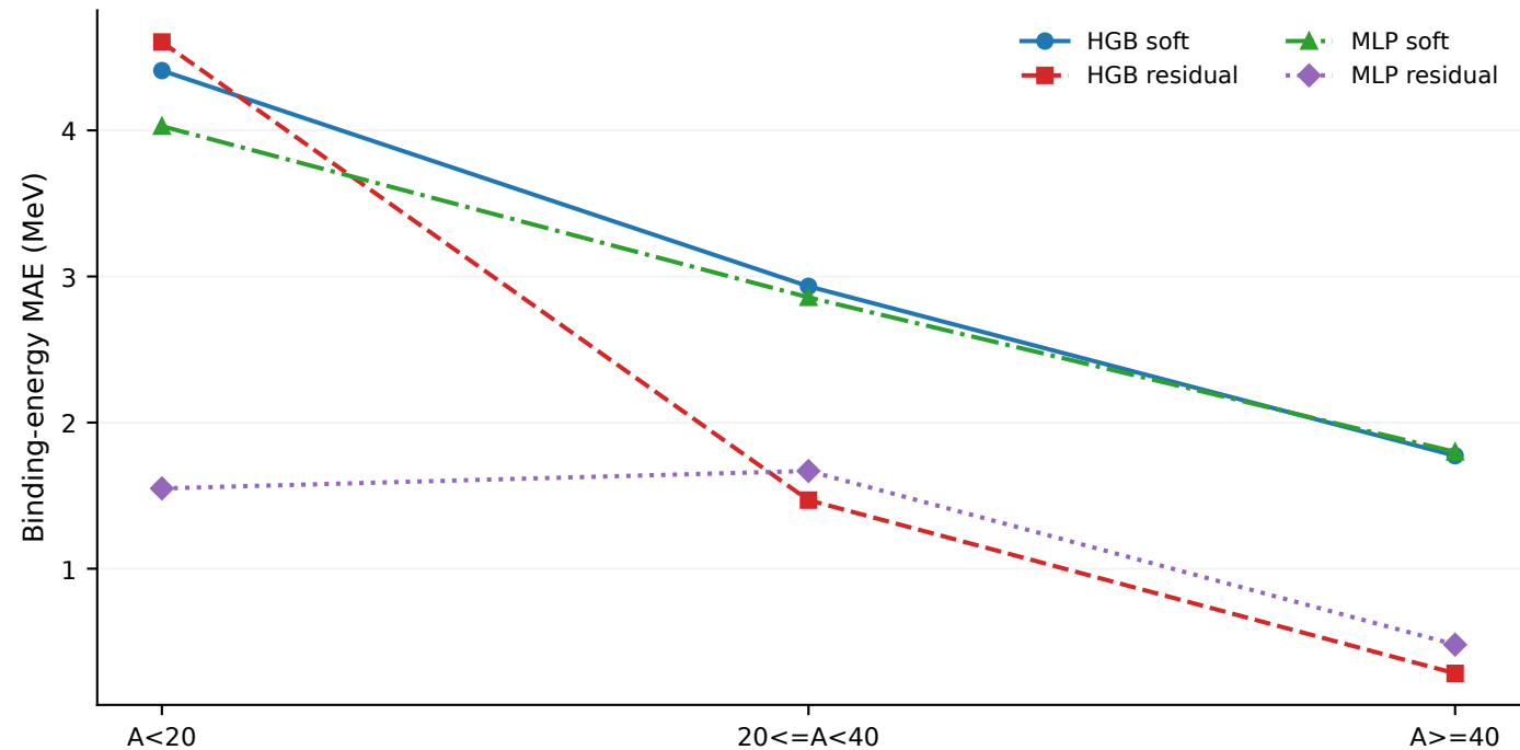
Supplementary light-nucleus model-validity stress test
