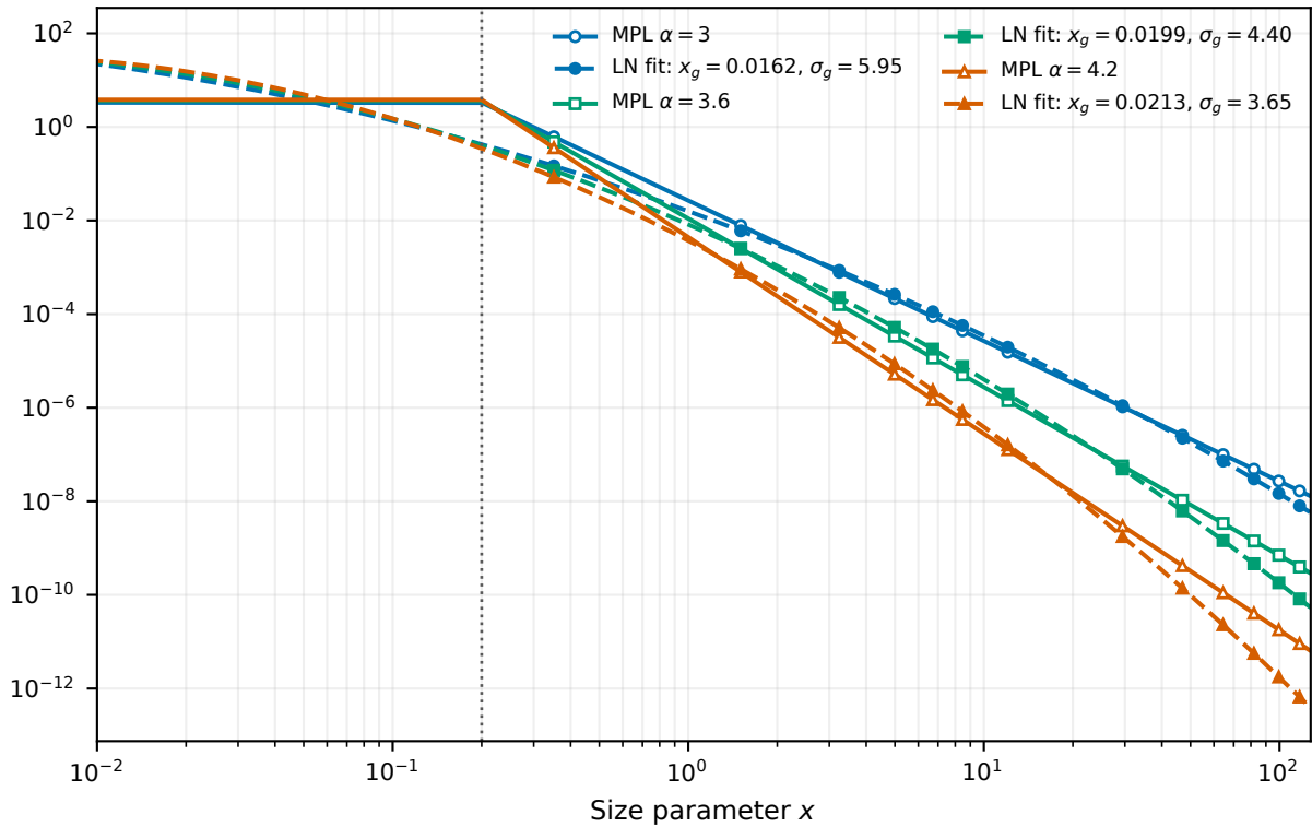
Normalized number density n(x)
