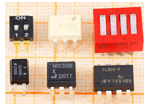
(c) Entegre devre
