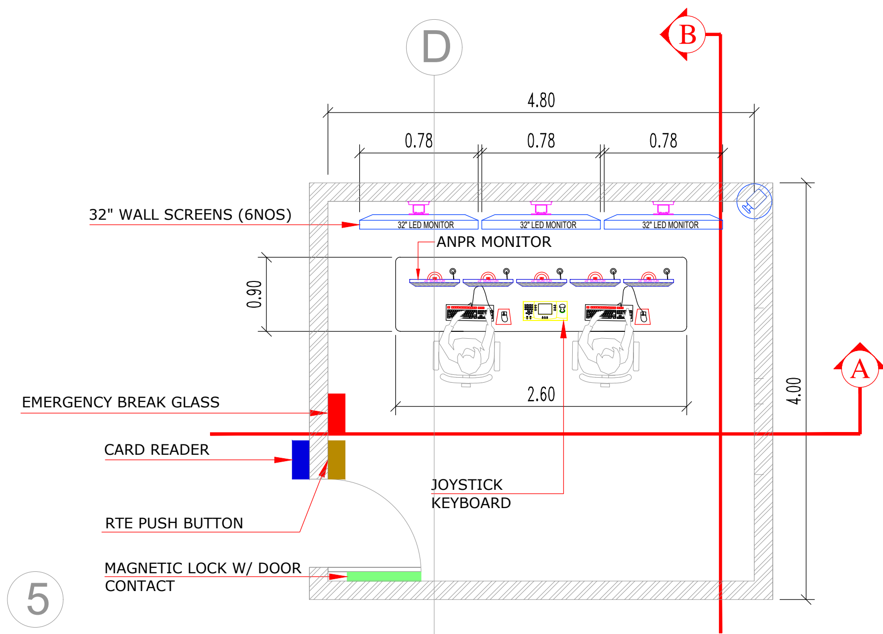
CONTROL ROOM FLOOR PLAN LOCATED AT SITE PLAN LAYOUT SCALE 1:25
