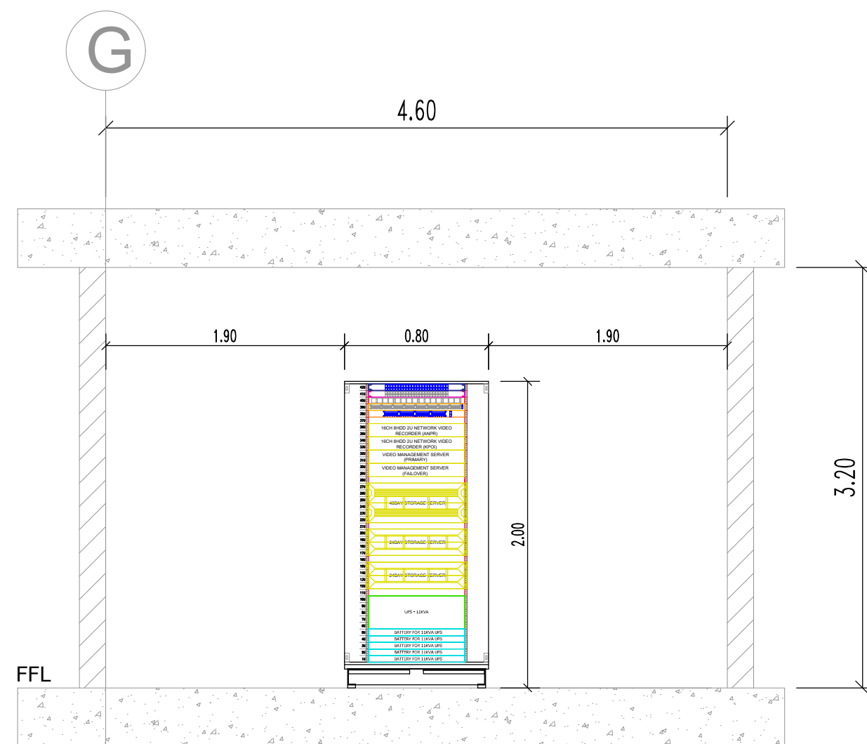
SECTION A-A (FRONT VIEW) SCALE 1:25
