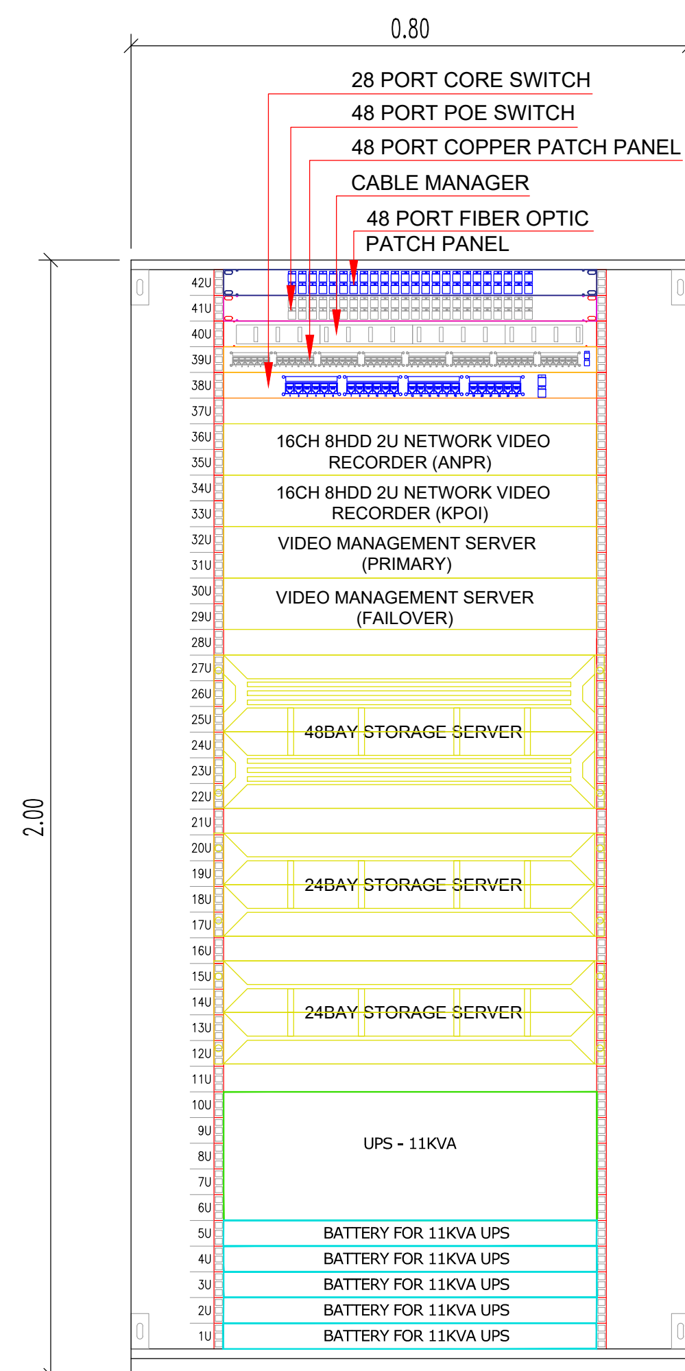
MAIN EQUIPMENT RACK (MDF) - 42U DETAILED VIEW
