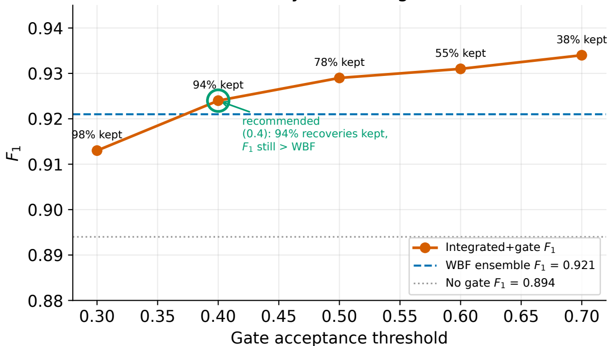
Precision gate: a recovery-vs- F_1 dial (labels = fraction of beyond-ceiling recoveries retained)
