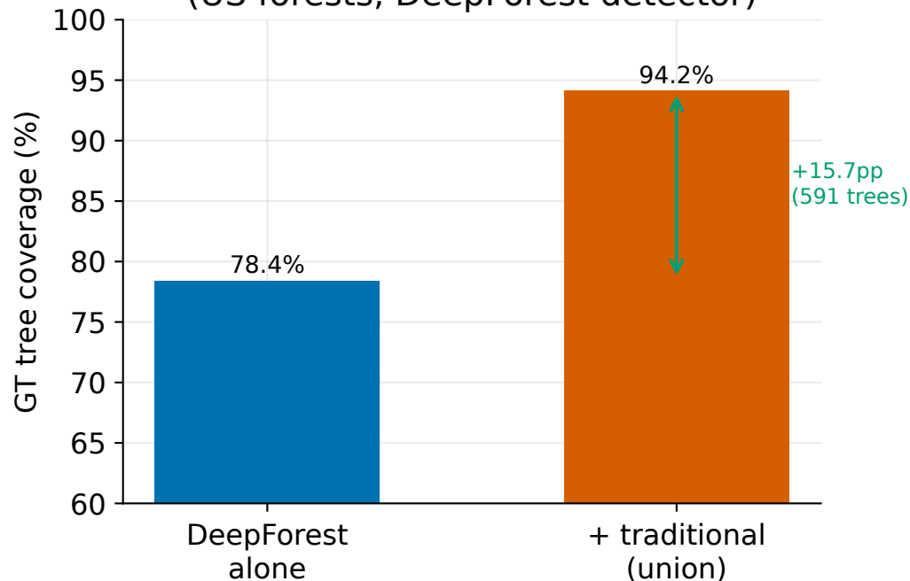
Beyond-ceiling recovery on NEON (US forests, DeepForest detector)
