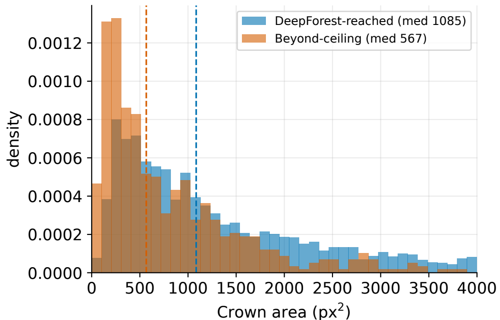
Recovered crowns are 1.9× smaller (same mechanism as VHRTrees)
