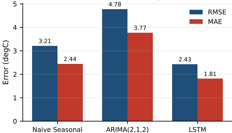
Phase-1 baseline comparison
