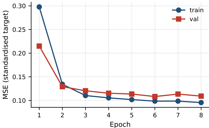
LSTM training curves
