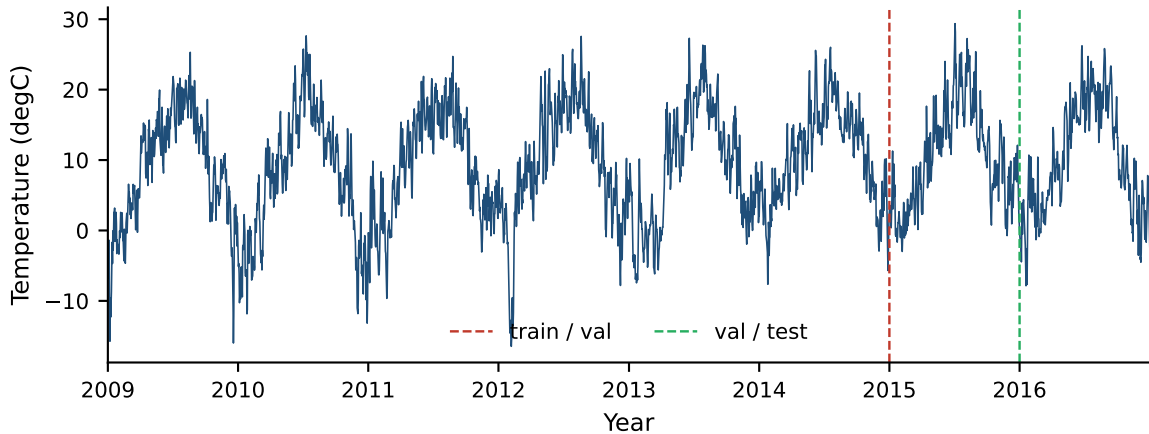
Jena Climate -- daily mean of T (degC)
