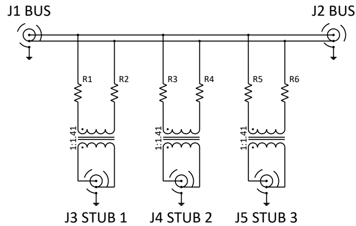
SCHEMATIC DIAGRAM
