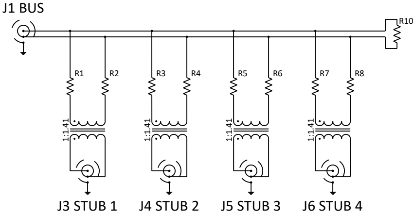
SCHEMATIC DIAGRAM
