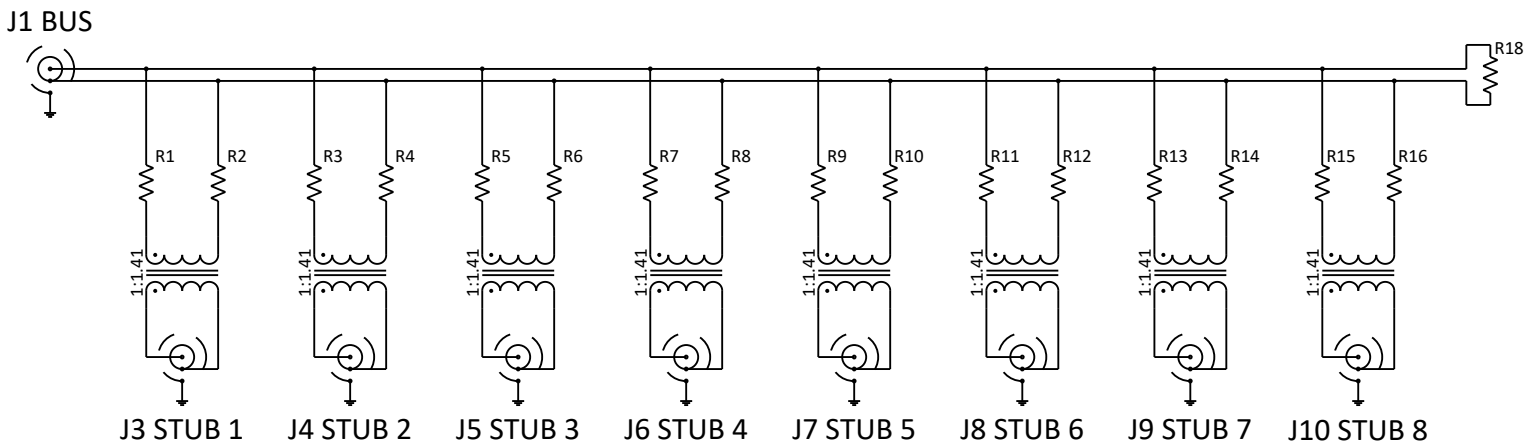
SCHEMATIC DIAGRAM
