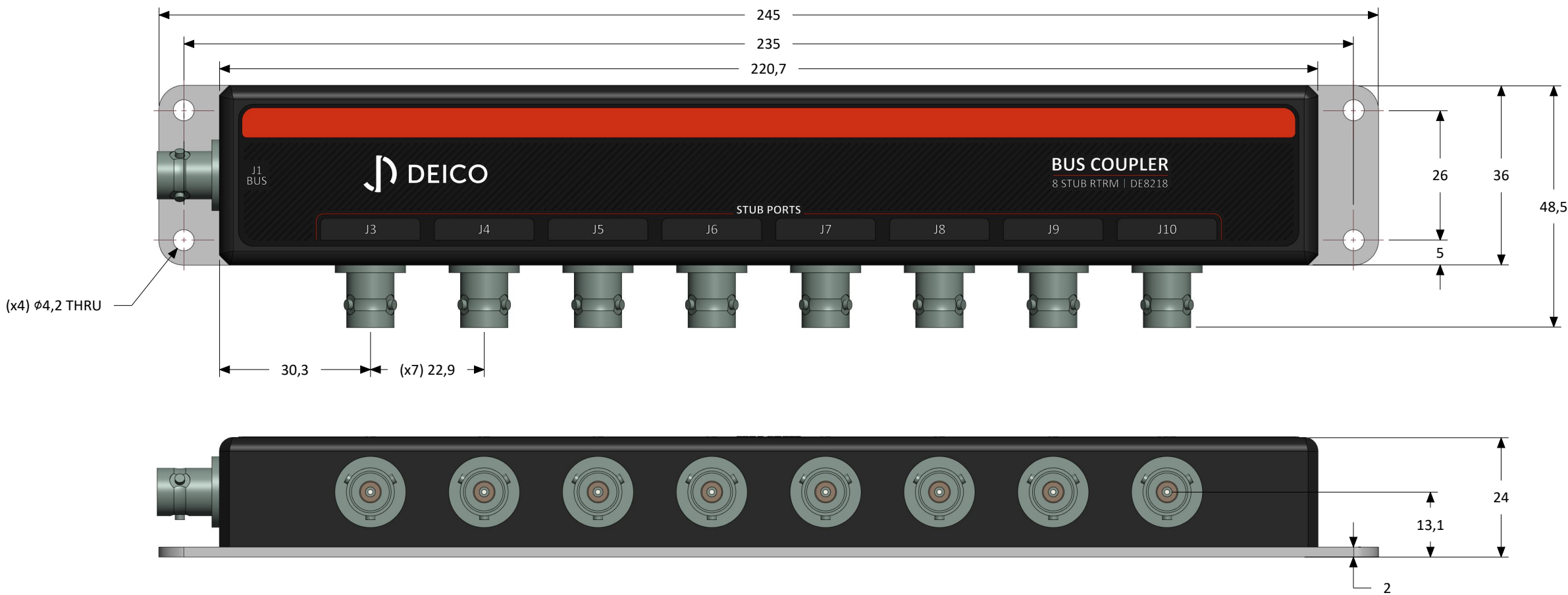
SCHEMATIC DIAGRAM
