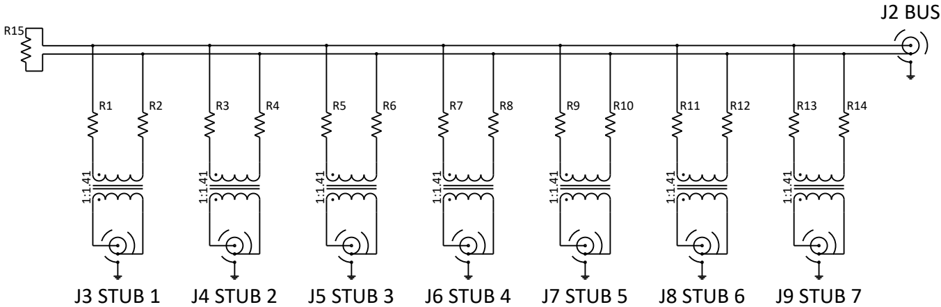
SCHEMATIC DIAGRAM
