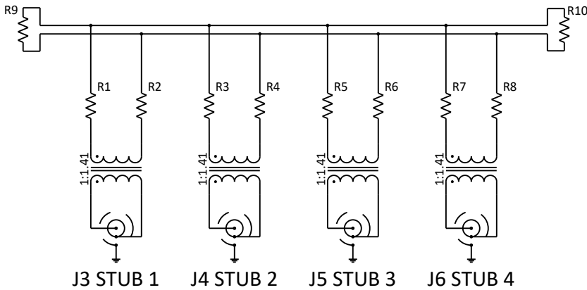
SCHEMATIC DIAGRAM
