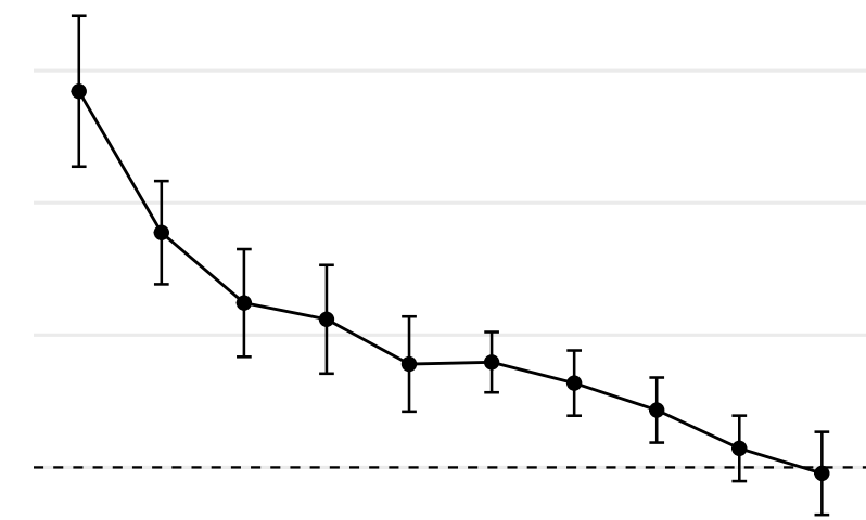
Out-of-state high schools
