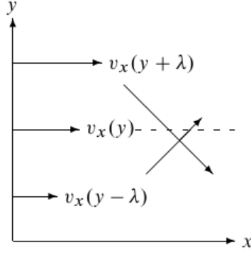
Figure 27: Layers of gas moving with different velocities give rise to shear forces because they exchange molecules with different average velocities. Figure taken from Ref. [3].
