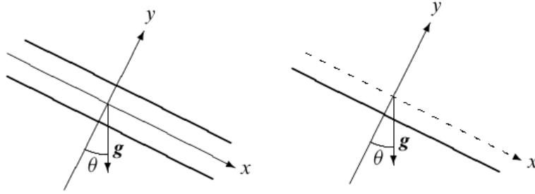
Figure 30: Left: Parallel plates inclined an angle \theta to the horizon. Right: Flow with an open surface on a plate inclined an angle \theta to the horizon. Figures taken from Ref. [3].
