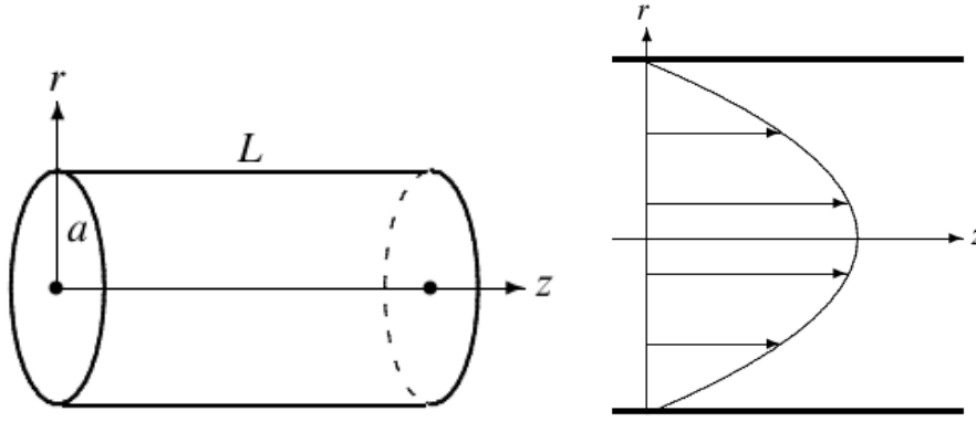
Figure 32: Left: Section of a circular pipe of inner radius a and length L . The pressure is higher at z = 0 than at z = L , and the pressure drop \Delta p = p(0) - p(L) drives the fluid through the pipe. Right: Velocity profile for laminar flow through a circular pipe. Figures taken from Ref. [3].
