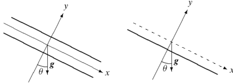
Figure 31: Left: Parallel plates inclined an angle \theta to the horizon. Right: Flow with an open surface on a plate inclined an angle \theta to the horizon. Figures taken from Ref. [3].
