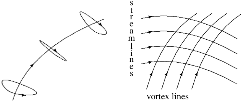
Figure 10: Left: Around a vortex line there is local circulation of fluid. Right: The Bernoulli field is constant on surfaces made from vortex lines and streamlines.
