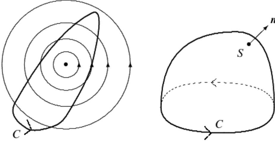
Figure 11: Left: A closed curve C encircling a whirl. Right: A surface S with perimeter C . The normal to the surface is consistent with the orientation of C (here using a right-hand rule).
