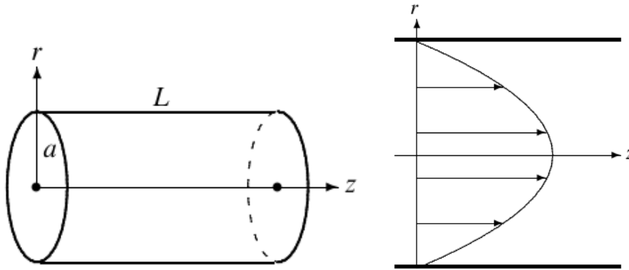
Figure 19: Left: Section of a circular pipe of inner radius a and length L . The pressure is higher at z = 0 than at z = L , and the pressure drop \Delta p = p(0) - p(L) drives the fluid through the pipe. Right: Velocity profile for laminar flow through a circular pipe. Figures taken from Ref. [3].
