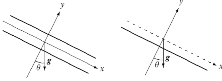
Figure 18: Left: Parallel plates inclined an angle \theta to the horizon. Right: Flow with an open surface on a plate inclined an angle \theta to the horizon. Figures taken from Ref. [3].
