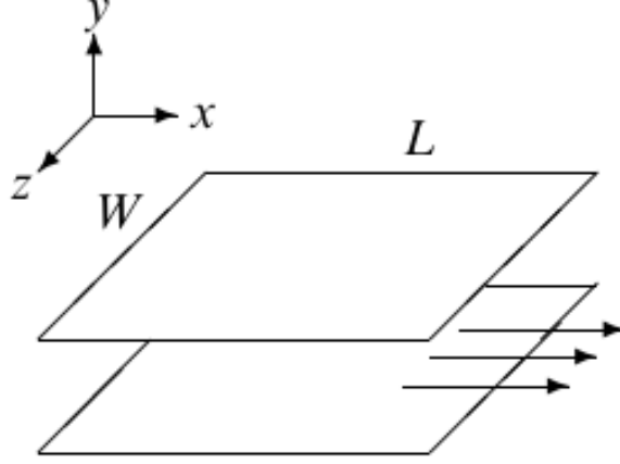
Figure 16: Channel flow between plates of width W parallel and length L . Figure taken from Ref. [3].
