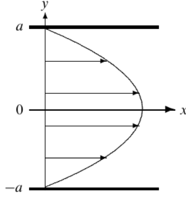
Figure 17: Characteristic parabolic steady velocity profile between the infinitely extended plates with distance d = 2a . Figure taken from Ref. [3].
