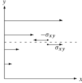
Figure 14: Shear viscosity in laminar (layered) flow. The fluid above the dashed line moves slightly faster than the fluid below and exerts a positive shear stress \sigma_{xy} on the fluid beneath. By Newton's third law, the fluid below exerts an opposite shear stress -\sigma_{xy} on the fluid above. Figure taken from Ref. [3].
