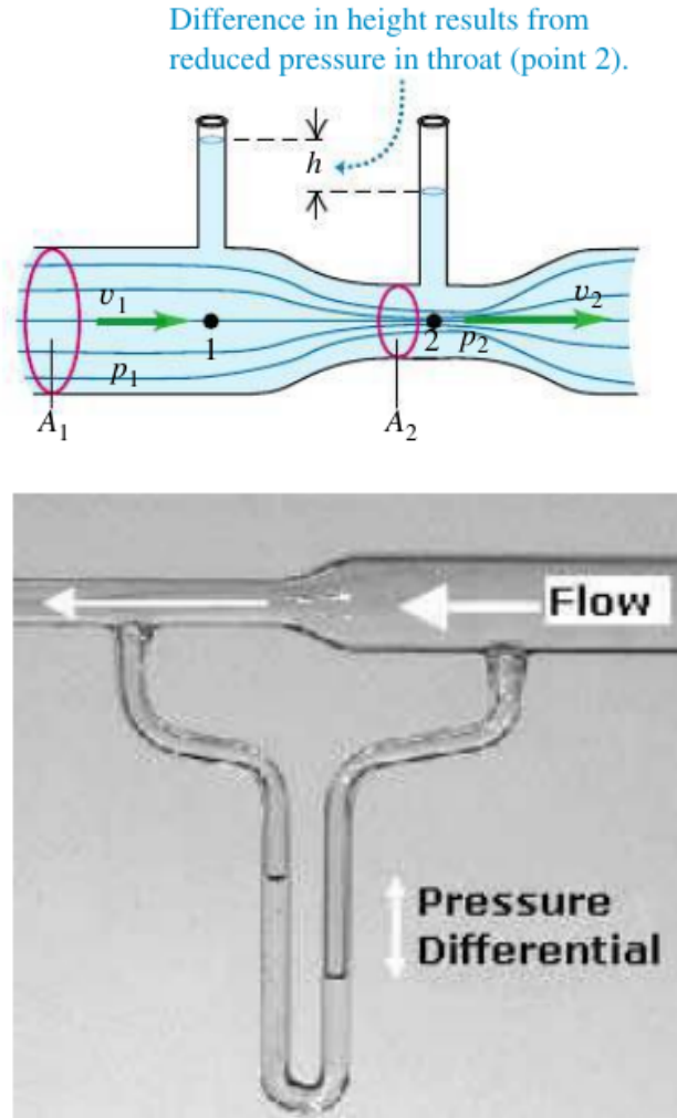
Figure 7: Top: The Venturi meter is used to measure flow speed in a pipe. Bottom: Venturi effect demonstration. Air streams from the right into a narrower tube where it speeds up. The shift in water level in the shunt tube underneath can be used to determine the pressure drop and thus the flow speed.
