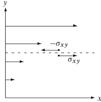
Figure 23: Shear viscosity in laminar (layered) flow. The fluid above the dashed line moves slightly faster than the fluid below and exerts a positive shear stress \sigma_{xy} on the fluid beneath. By Newton’s third law, the fluid below exerts an opposite shear stress -\sigma_{xy} on the fluid above. Figure taken from Ref. [3].
