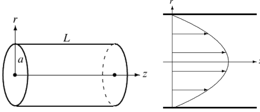
Figure 28: Left: Section of a circular pipe of inner radius a and length L . The pressure is higher at z = 0 than at z = L , and the pressure drop \Delta p = p(0) - p(L) drives the fluid through the pipe. Right: Velocity profile for laminar flow through a circular pipe. Figures taken from Ref. [3].
