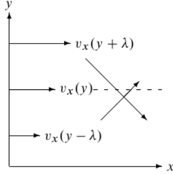
Figure 24: Layers of gas moving with different velocities give rise to shear forces because they exchange molecules with different average velocities. Figure taken from Ref. [3].
