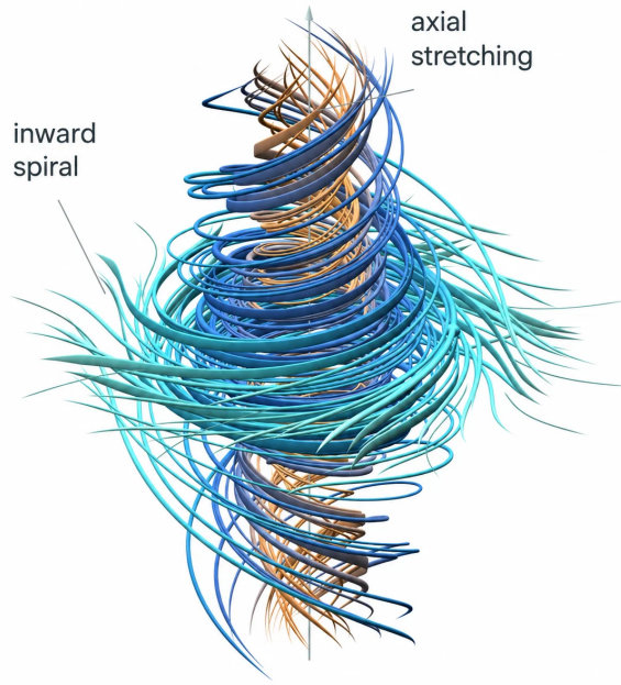
Figure 30: A snapshot of local incompressible motion. Orange marks faster angular rotation; teal marks slower rotation. Circulating speed also depends on radius. The trajectories show inward spiraling and axial stretching. Figure taken from OpenAI webpage.
