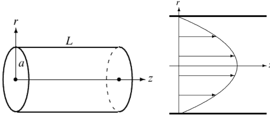
Figure 34: Left: Section of a circular pipe of inner radius a and length L . The pressure is higher at z = 0 than at z = L , and the pressure drop \Delta p = p(0) - p(L) drives the fluid through the pipe. Right: Velocity profile for laminar flow through a circular pipe. Figures taken from Ref. [3].
