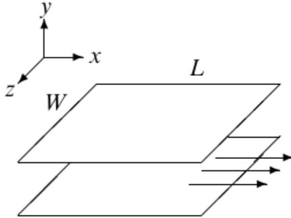
Figure 31: Channel flow between plates of width W parallel and length L . Figure taken from Ref. [3].
