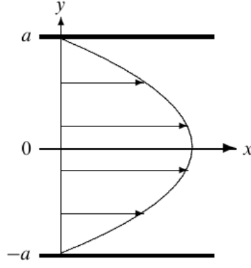
Figure 32: Characteristic parabolic steady velocity profile between the infinitely extended plates with distance d = 2a . Figure taken from Ref. [3].
