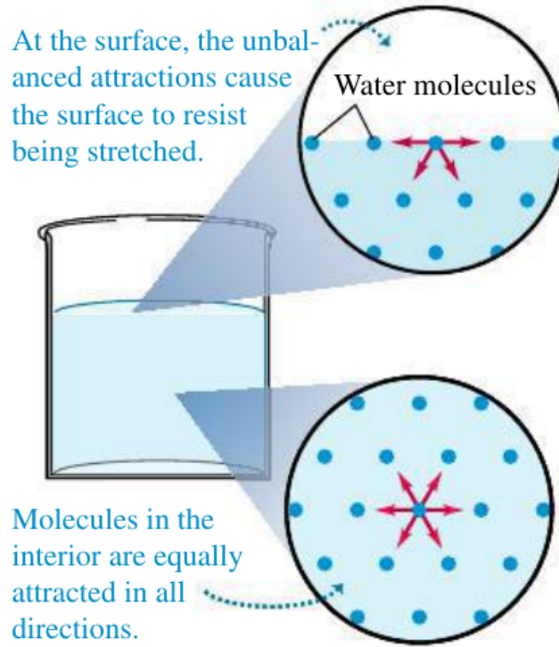
Figure 45: A molecule at the surface of a liquid is attracted into the bulk liquid, which tends to reduce the liquid's surface area. Figure taken from Ref. [6].
