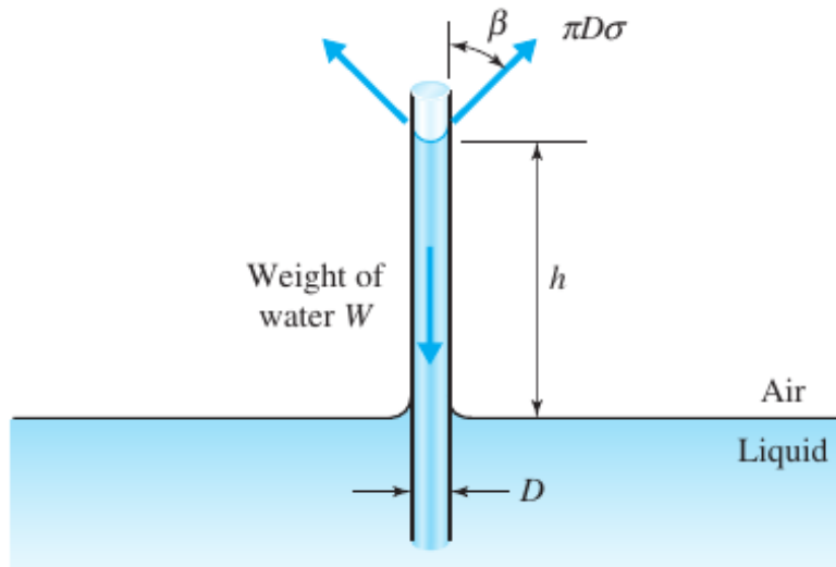
Figure 56: Rise in a capillary tube. Figure taken from Ref. [4].
