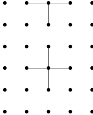
Figure 47: Cross-section of a primitive three-dimensional model of a material interfacing to vacuum. A molecule at the surface has only five bonds compared to the six that link a molecule in the interior. The missing bond energy at the surface gives rise to a positive surface energy density, which is the cause of surface tension. Figure taken from Ref. [3].
