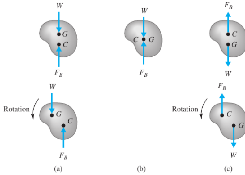
Figure 42: Stability of a submerged body: (a) unstable; (b) neutral; (c) stable. Figure taken from Ref. [4].
