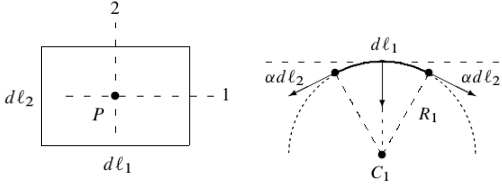
Figure 53: Left: Tiny rectangle aligned with the principal directions, seen from “above”. The sides are d\ell_1 and d\ell_2 . Right: The rectangular piece of the surface with sides d\ell_1 and d\ell_2 is subject to two tension forces along the 1-direction resulting in a normal force pointing toward the center of curvature C_1 . The tension forces in the 2-direction contribute analogously to the normal force. Figure taken from Ref. [3].
