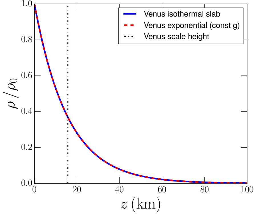
Figure 20: Isothermal slab model applied to Venus. The difference between the full expression and an exponential profile is negligible. In this case, M \approx 0.815 M_{\oplus} , R \approx 0.95 R_{\oplus} , and p_0 \approx 93 \times 10^5 Pa, leading to x \approx 70 \gg 1 .
