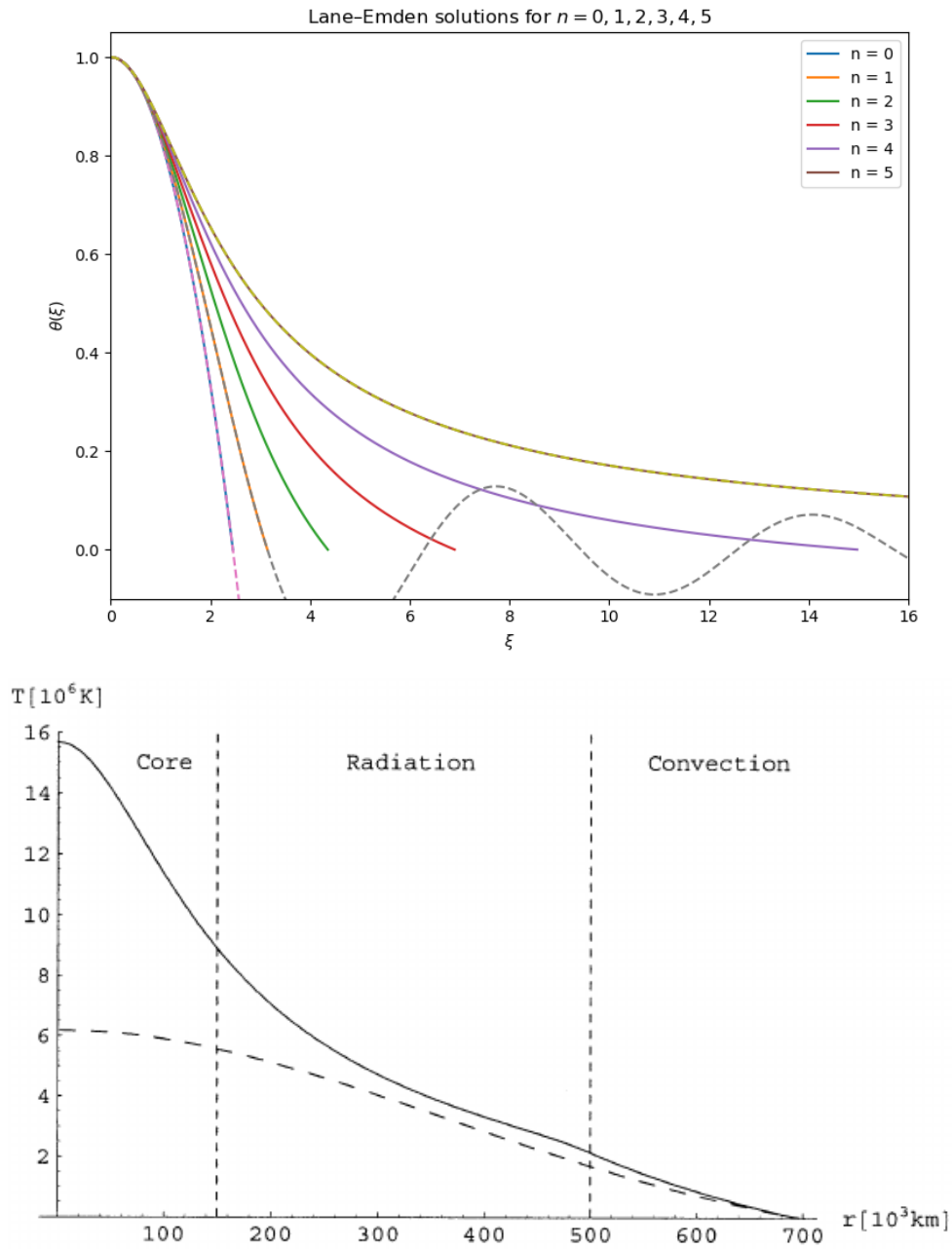
Figure 22: Top: Solutions to the Lane-Emden equation for various values of n . The higher n , the larger the \xi value for which the solution crosses \theta = 0 . Bottom: The temperature distribution in the Sun as a function of the distance from the centre. The fully drawn curve is from the ‘standard’ Sun model and the dashed curve is the Lane-Emden solution for \gamma = 5/3 .
