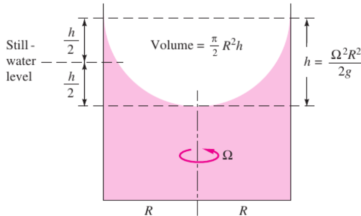
Figure 30: Determining the free-surface position for rotation of a cylinder of fluid about its central axis. Figure taken from [5].
