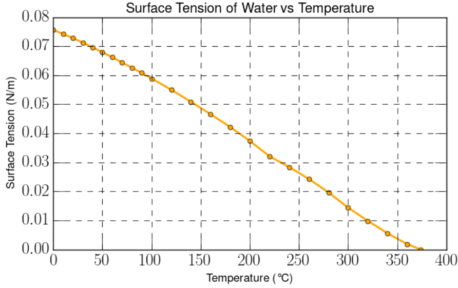
Figure 46: Surface tension of a clean air–water interface. Data from Table 7.
