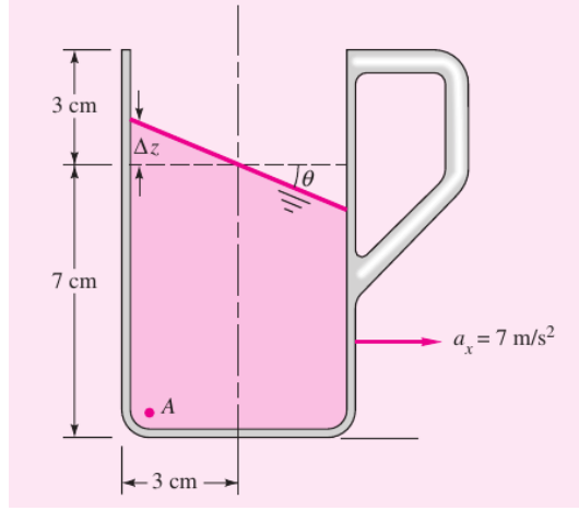
Figure 28: The coffee tilted during the acceleration. Figure taken from [5].
