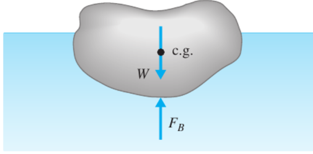
Figure 34: Forces on a floating object. Figure taken from Ref. [4].
