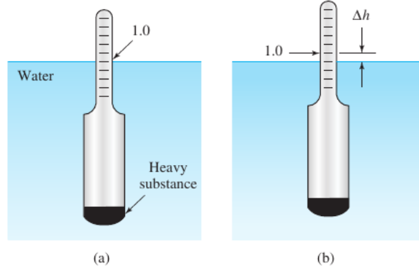
Figure 35: Hydrometer: (a) in water; (b) in an unknown liquid. Figure taken from Ref. [4].
