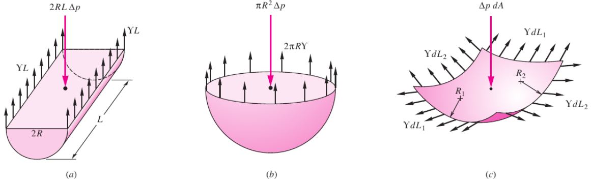
Figure 48: Pressure change across a curved interface due to surface tension (here denoted as \Upsilon ): (a) interior of a liquid cylinder; (b) interior of a spherical droplet; (c) general curved interface. Figure taken from Ref. [5].
