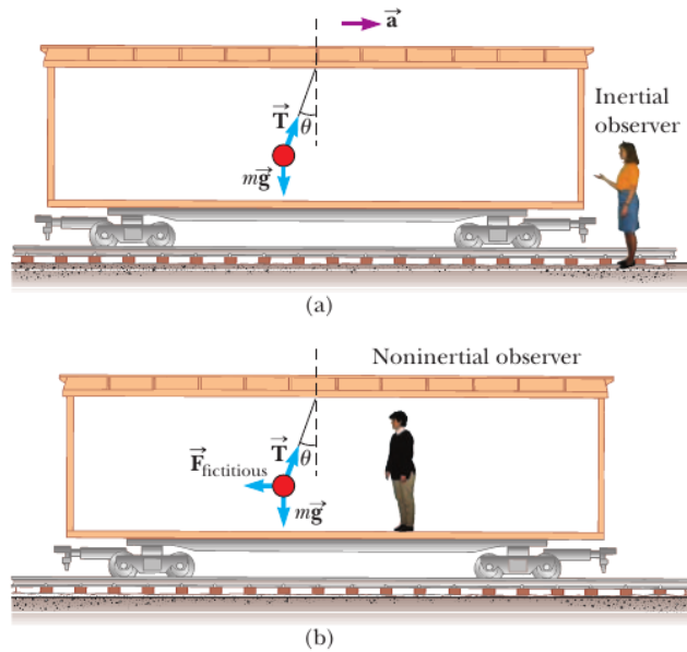
Figure 24: A small sphere suspended from the ceiling of a boxcar accelerating to the right is deflected as shown. (a) An inertial observer at rest outside the car claims that the acceleration of the sphere is provided by the horizontal component of \vec{T} . (b) A noninertial observer riding in the car says that the net force on the sphere is zero and that the deflection of the cord from the vertical is due to a fictitious force \vec{T}_{\text{fictitious}} that balances the horizontal component of \vec{T} . Figure taken from Ref. [8].
