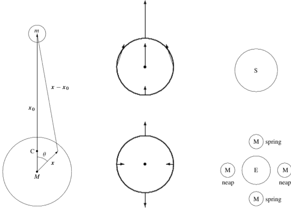
Figure 32: Left: geometry of the Earth and the Moon (not to scale). The point C is the center of mass of the system. Center: (top) how the Moon's gravity varies over the Earth (exaggerated); (bottom) the Moon's gravity with the unobservable constant acceleration canceled. This figure explains why the tides have a semi-diurnal period. Right: Earth and Sun with the Moon in extreme positions corresponding to spring tides and neap tides. The figure is (vastly) not to scale. Figures taken from Ref. [3].
