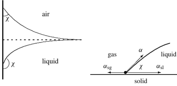
Figure 55: Fig. 1.12 Contact-angle effects at liquid-gas-solid interface. If \theta < 90^\circ , the liquid “wets” the solid; if \theta > 90^\circ , the liquid is nonwetting. Figure taken from Ref. [5].
