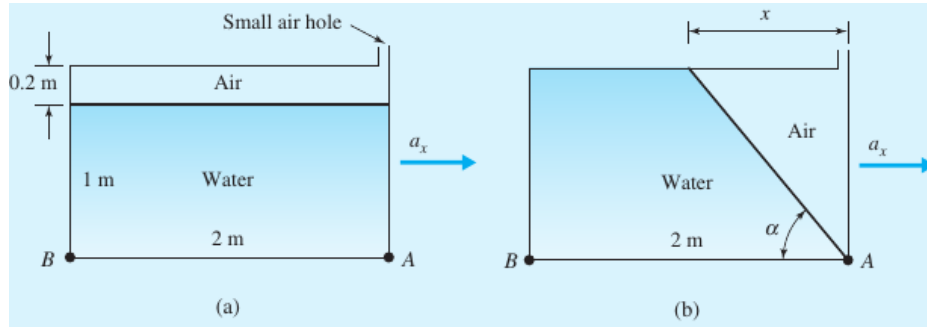
Figure 27: Linearly accelerating tank. Figure taken from [4].
