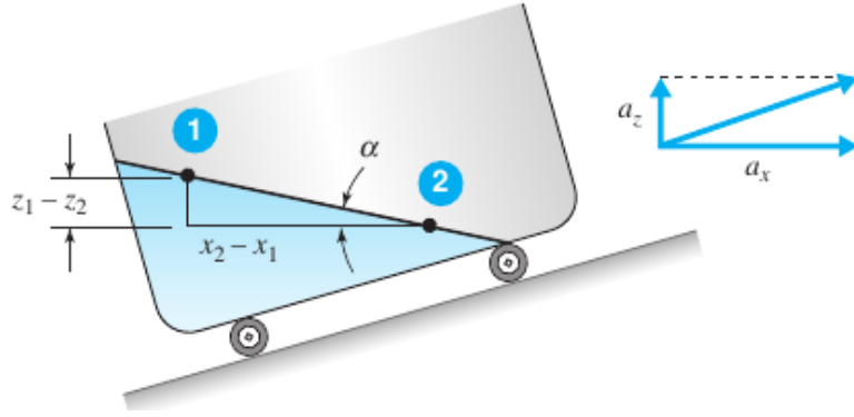
Figure 26: Linearly accelerating container. Figure taken from [4].
