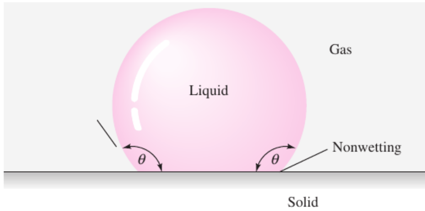
Figure 54: Contact-angle effects at liquid–gas–solid interface. If \theta < 90^\circ , the liquid “wets” the solid; if \theta > 90^\circ , the liquid is nonwetting. Figure taken from Ref. [5].
