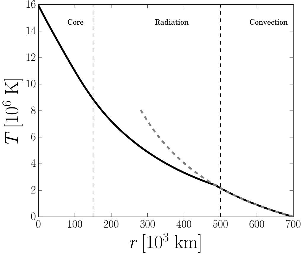
Figure 11: The temperature distribution in the Sun as a function of the distance from the center. The vertical lines are boundaries between the three major layers of the Sun. The fully drawn curve is an approximate fit to the solution from the Standard Sun model. The dashed curve is the approximative homentropic solution for the convective envelope.
