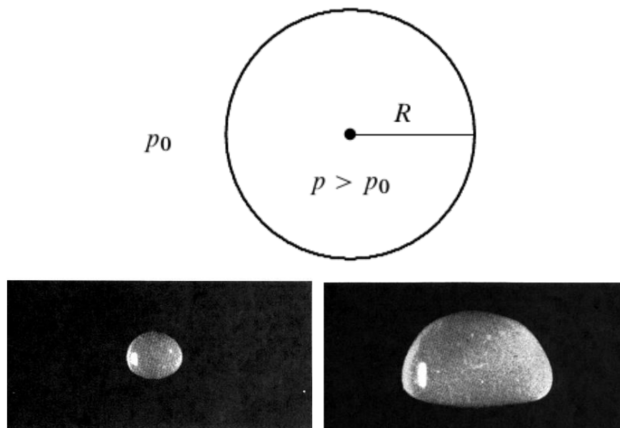
Figure 51: Top: Surface tension makes the pressure higher inside a spherical droplet or bubble. Bottom: Steadily falling raindrops are subject to the combined effects of surface tension, gravity, friction, and air currents. Left: Small raindrops are dominated by surface tension and therefore nearly spherical. Here the drop radius is slightly larger than the capillary length of 2.7 mm and the drop is slightly oval. Right: Larger raindrops assume a typical “hamburger” shape. Figure taken from Ref. [3].
