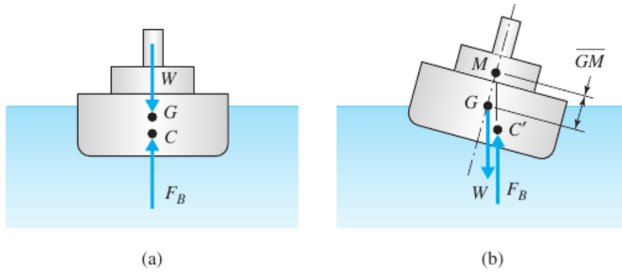
Figure 43: Stability of a floating body: (a) equilibrium position; (b) rotated position. Figure taken from Ref. [4].
