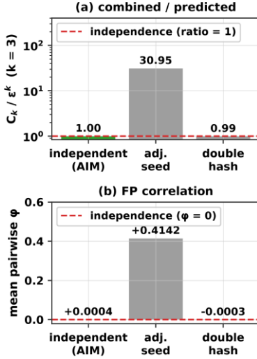
Fig. 3. Comparison of three hash configurations in terms of independence: (a) the ratio of the observed combined false positive rate to the independence prediction ( k=3 ; expected value 1), (b) the mean \phi correlation between filter pairs (expected value 0). Values represent the mean of five replicates; 95% confidence intervals are provided in the text.
