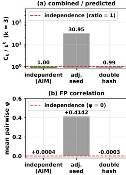
Fig. 4. Comparison of three hash configurations in terms of independence: (a) the ratio of the observed combined false positive rate to the independence prediction ( k = 3 ; expected value 1), (b) the mean \phi correlation between filter pairs (expected value 0). The setup on the left is the design used by AIM.
