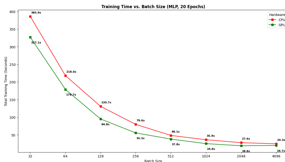
Figure 8. Training Time vs Batch Size.
