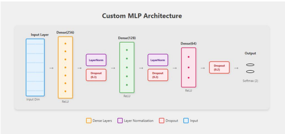
Figure 2. MLP Model Architecture.
