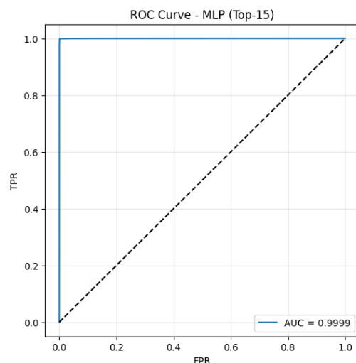
Figure 6. Test ROC Curve for the MLP Model.
