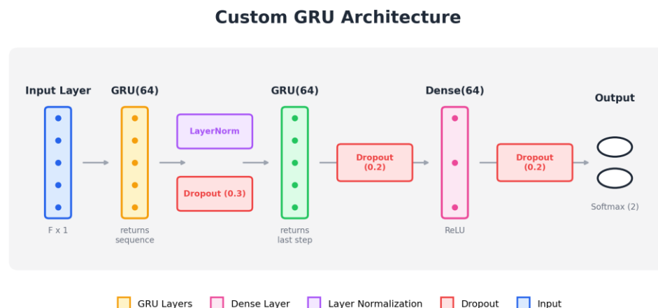
Figure 4. GRU Model Architecture.
