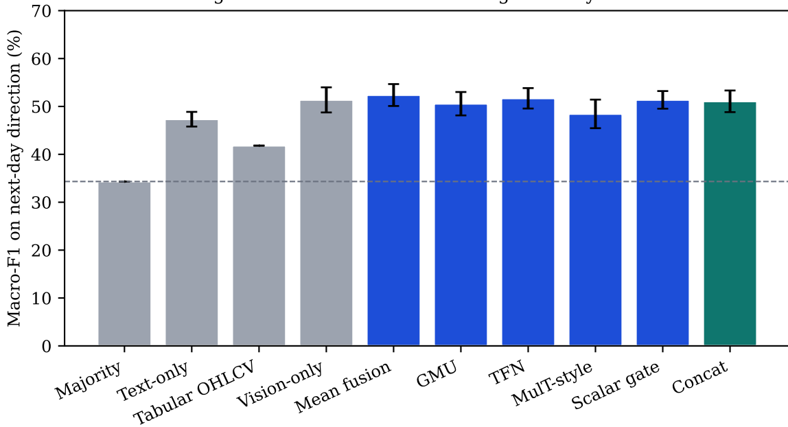
Leakage-free task: fusion does not significantly beat GMU
