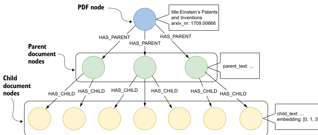
Figure 3.4 Parent document graph representation
