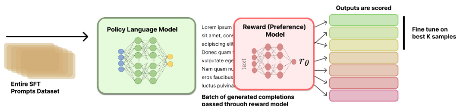
Figure 10.1 Rejection sampling overview.
