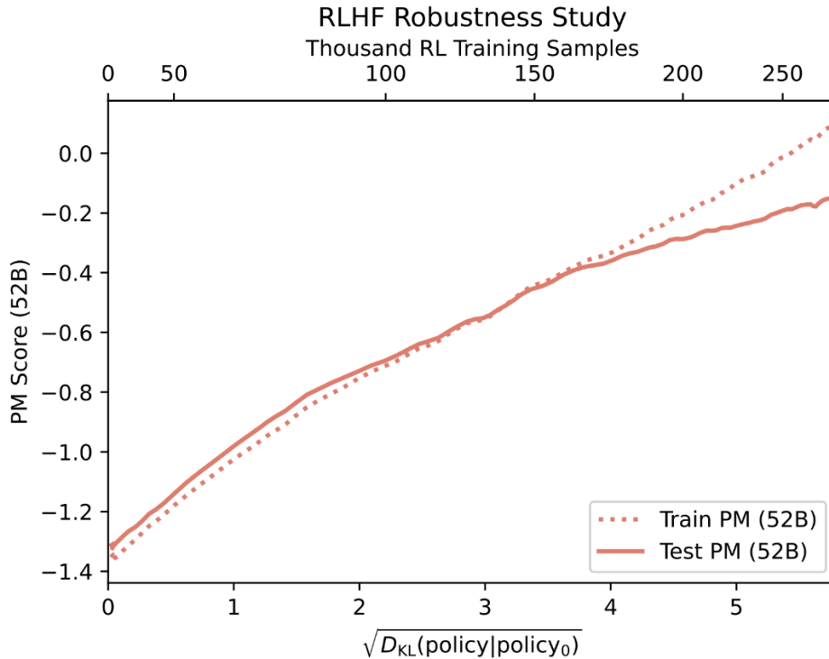
Figure 18.2 Over-optimization with a train and test RM from Bai et al. 2022. License CC-BY.
