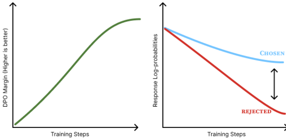
Figure 12.2 Sketch of preference displacement in DPO.
