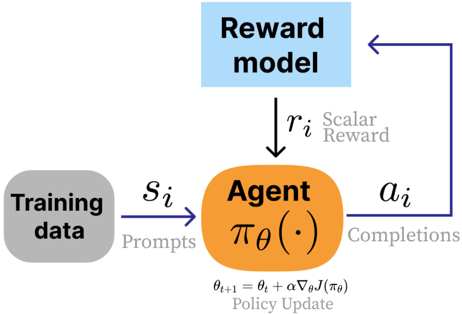
Figure 4.2 Standard RLHF loop
