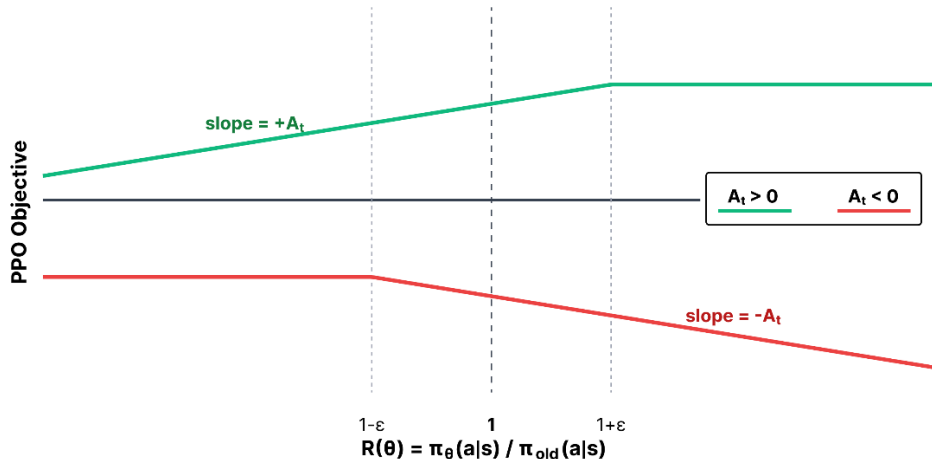
Figure 11.1 Visualization of the different regions of the PPO objective for a hypothetical advantage.
