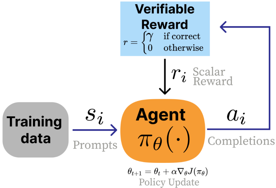
Figure 14.1 RLVR in the form of an RL feedback loop. Instead of a reward model, we use a verification function.
