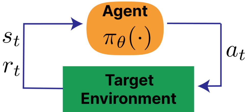
Figure 4.1 Standard RL loop
