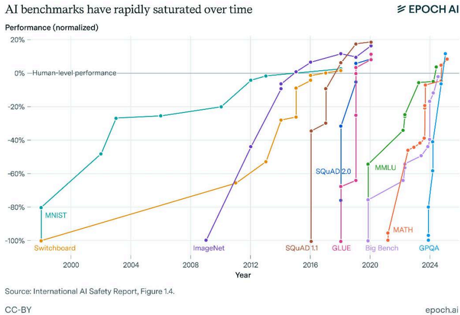
Figure 17.1 Report from Epoch AI showing how major AI evaluations are rapidly saturated over time. License CC-BY.
