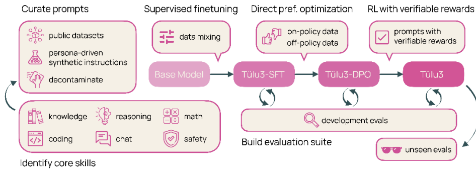
Figure 4.5 A summary of the Tulu 3 recipe with target skills and multi-step training recipe. Lambert et al. 2024, License CC-BY.
