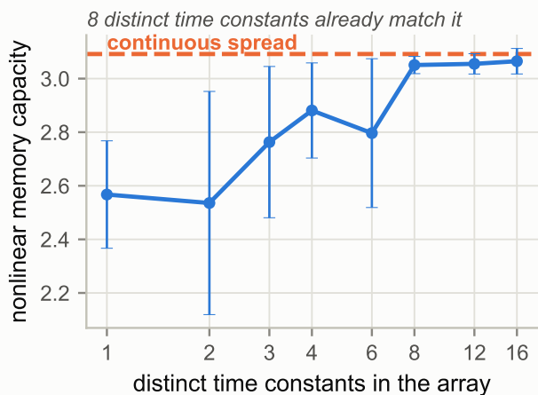
c How much of the spectrum is needed
