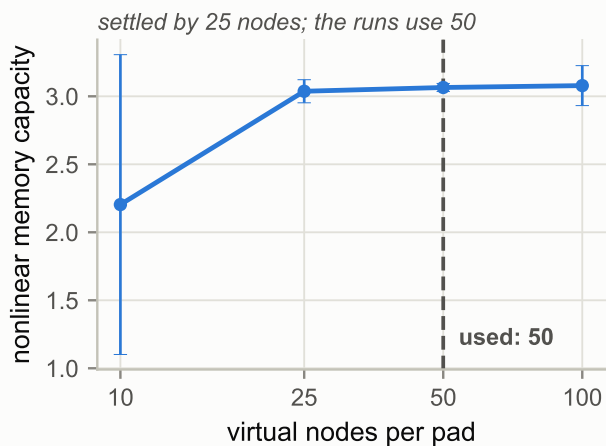
e Convergence: virtual nodes per pad
