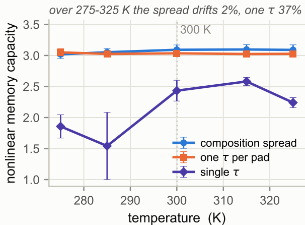
a Capacity against ambient temperature
