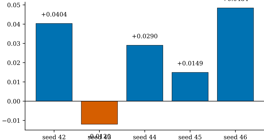
Per-seed regime gain of v4\_twostage over v3
