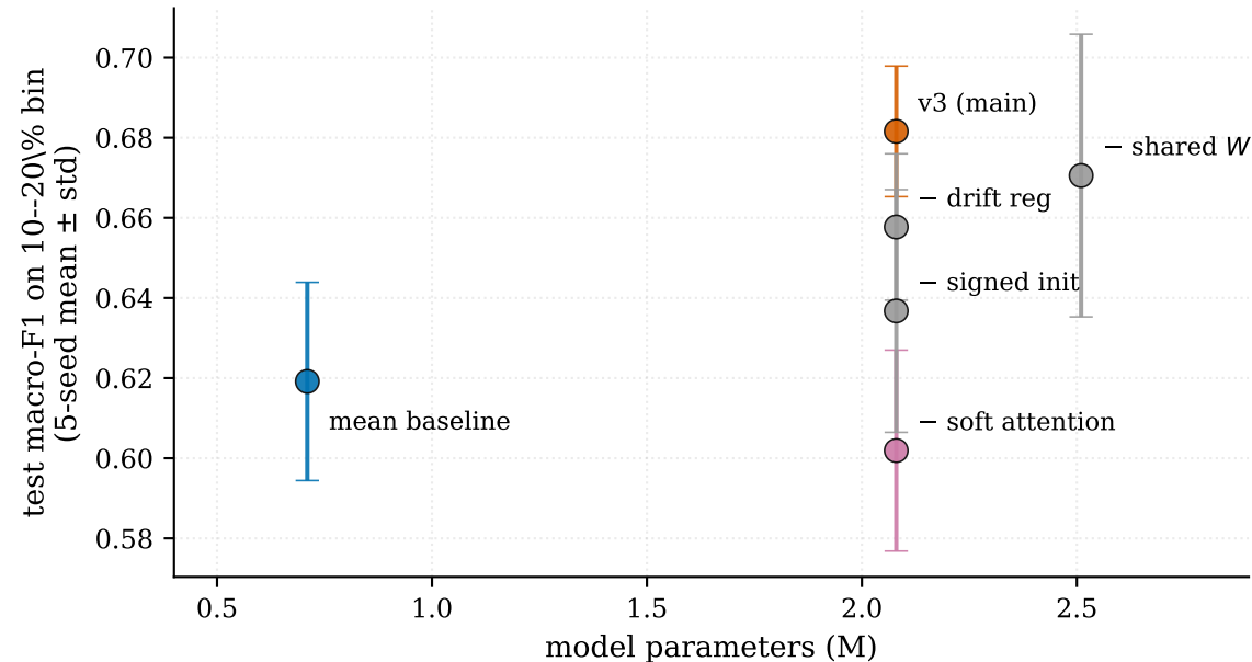
Compute-vs-gain on the operating regime
