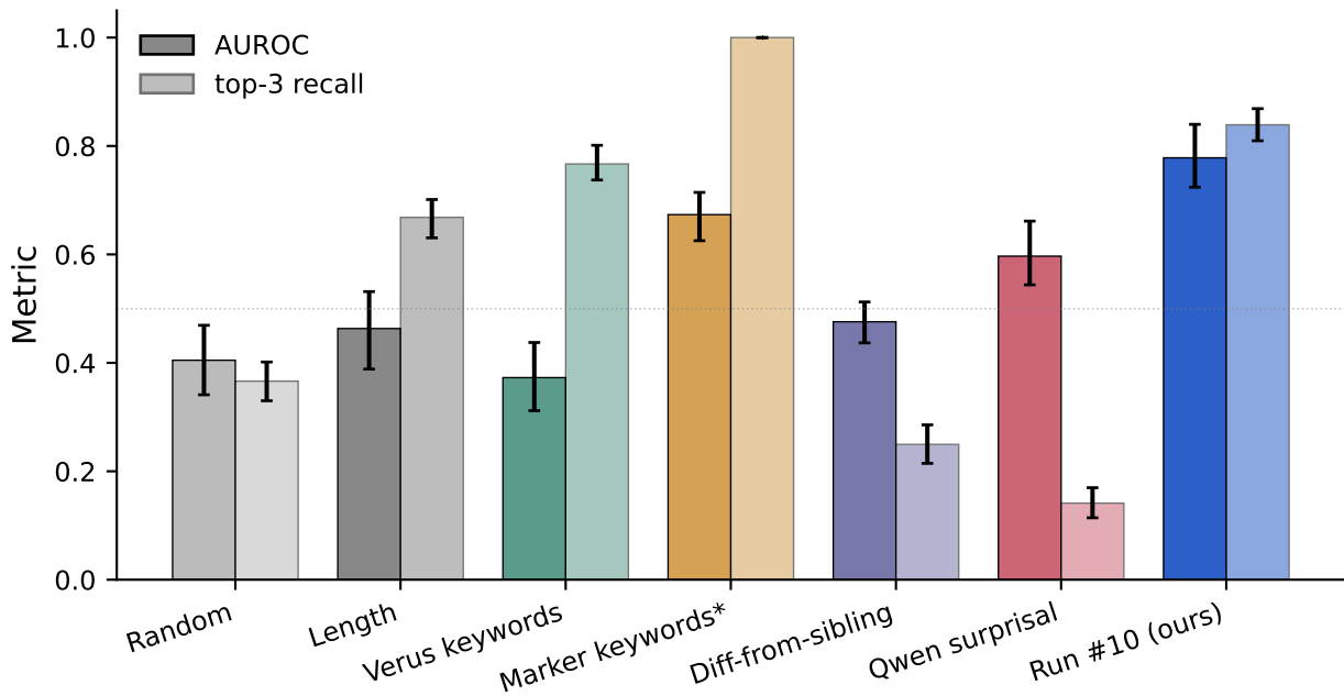
Baseline comparison on Verus dev-test corpus (n=1492)
