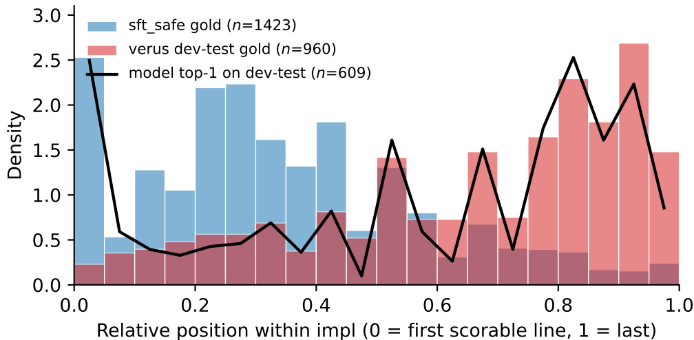
Buggy-line position shifts across corpora; model predictions track the dev-test distribution
