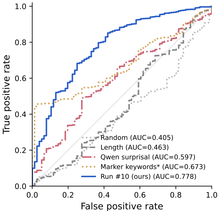
ROC: whole-impl FAIL vs PASS
