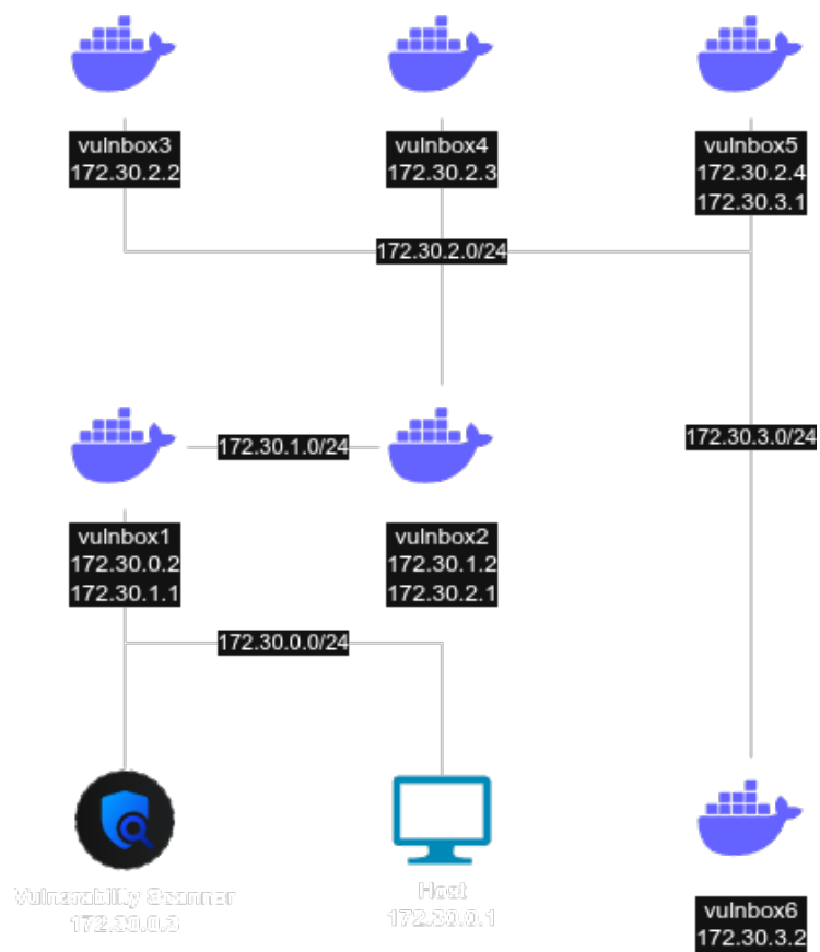
Figure 2.1: Network configuration
