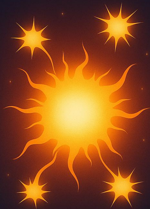
Nuclear fusion
