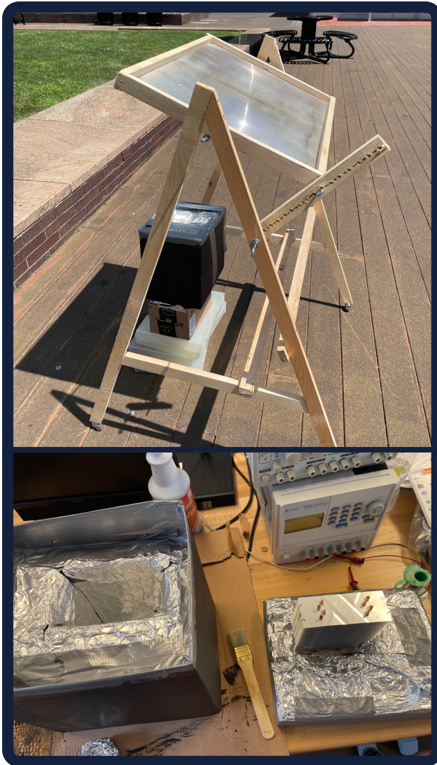
350F solar oven
