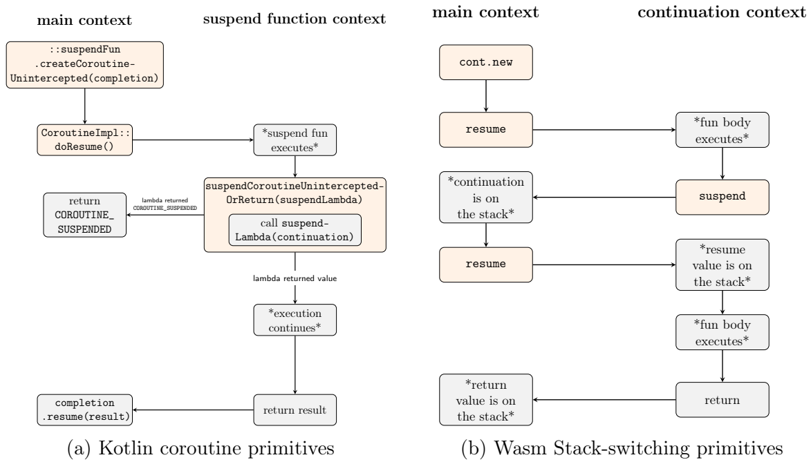
Figure 3.1: Comparison between Kotlin and Wasm coroutine primitives
