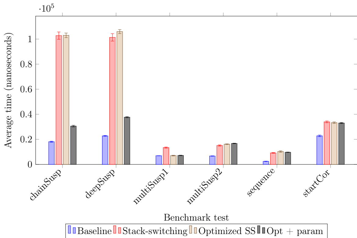
Figure 4.2: Benchmark comparison in dce mode, V8 runtime (error bars show 95% CI)
