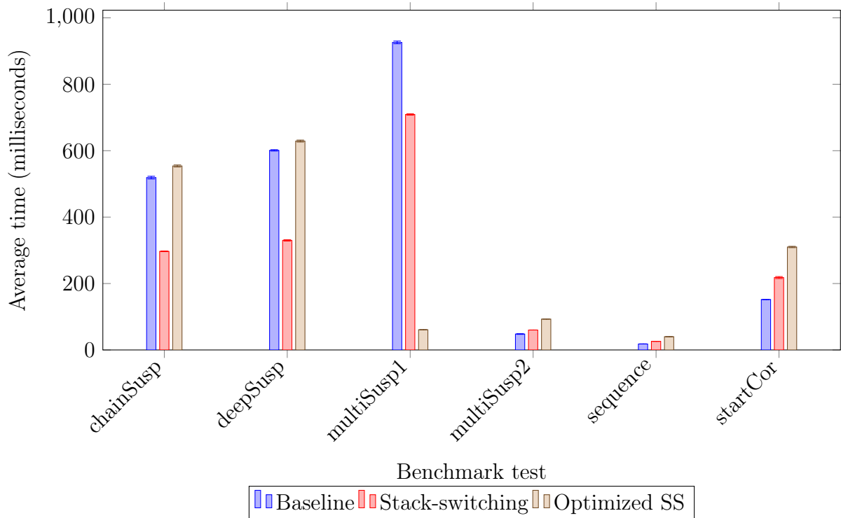
Figure 4.4: Benchmark comparison in dce mode, Reference Interpreter (error bars show 95% CI)
