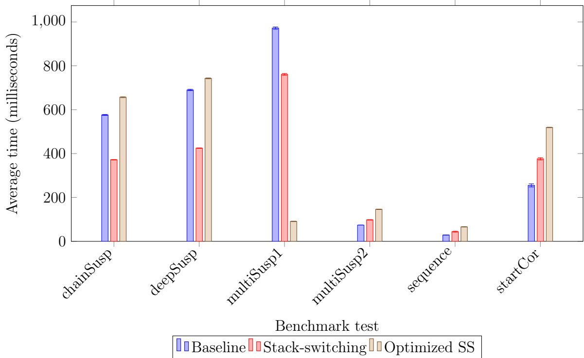
Figure 4.3: Benchmark comparison in dev mode, Reference Interpreter (error bars show 95% CI)
