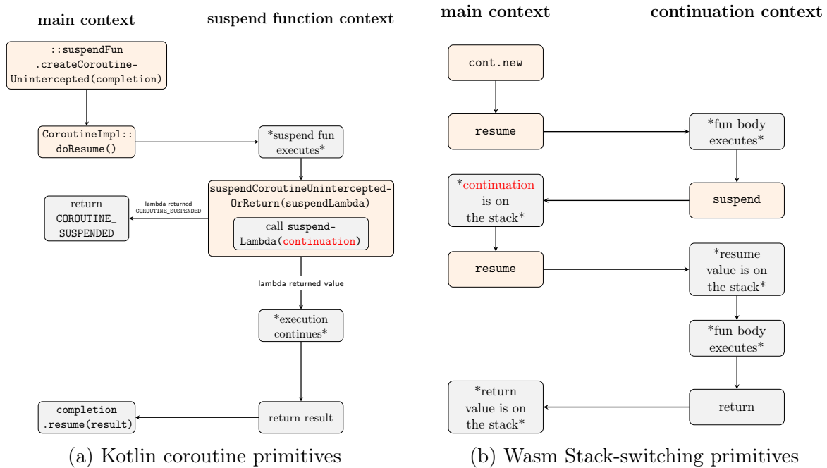
Figure 3.2: Continuation availability problem between Kotlin and Wasm
