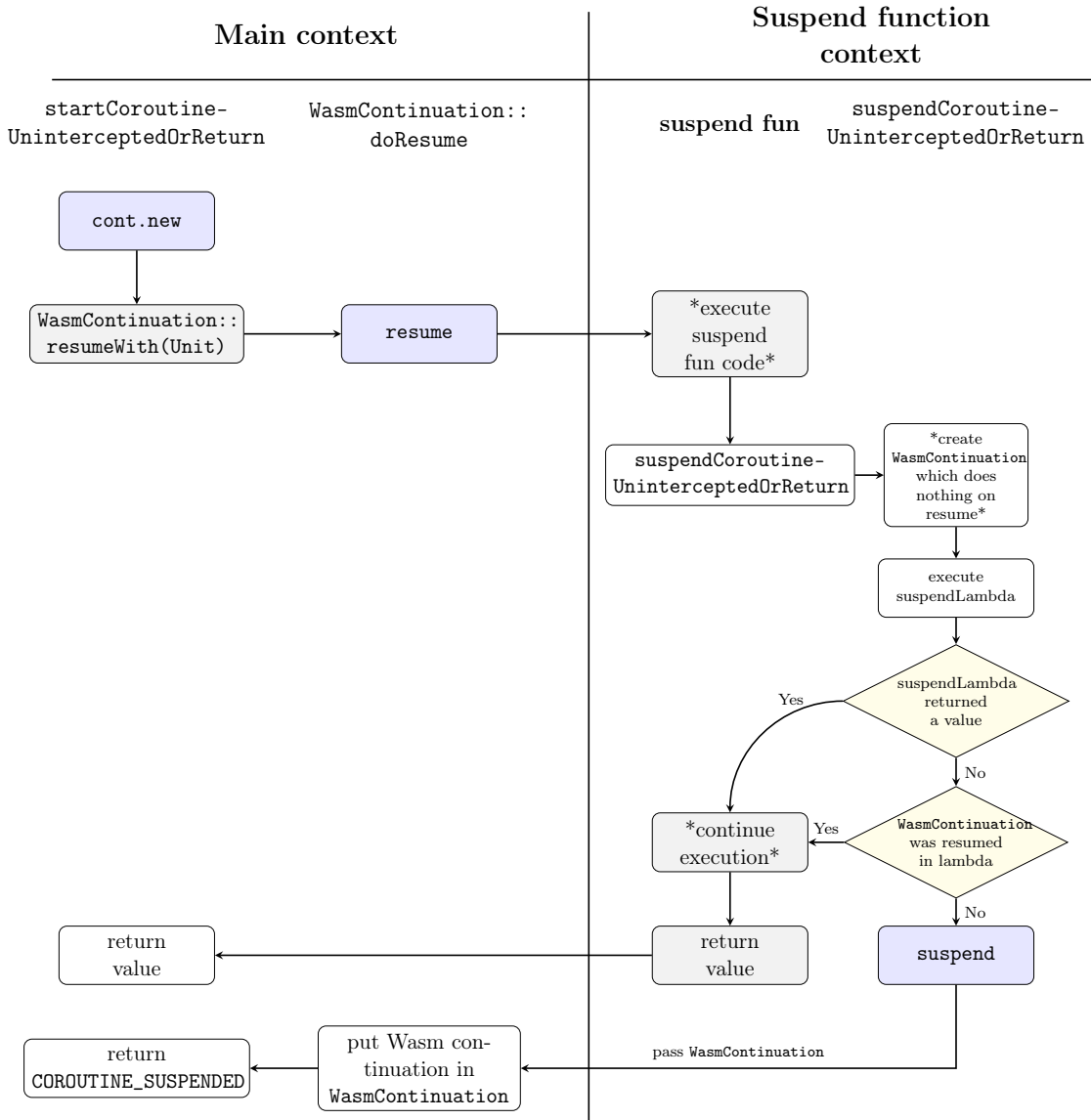
Figure 3.4: Immediate resume optimization
