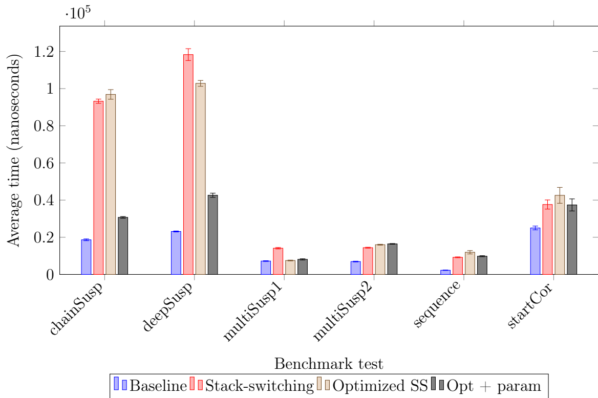
Figure 4.1: Benchmark comparison in dev mode, V8 runtime (error bars show 95% CI)
