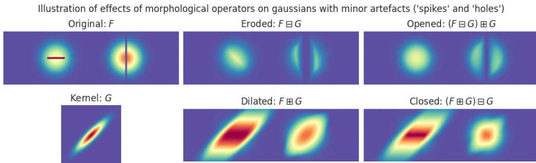
Figure 2.2: Illustration of an opening and closing, where warmer (red) colours indicate higher values and colder (blue) colours indicate lower values.
