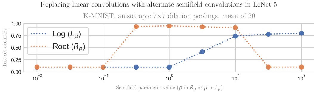
Figure 6.2: Results of nonlinear convolutions R_p and L_{\mu} for various p and \mu .
