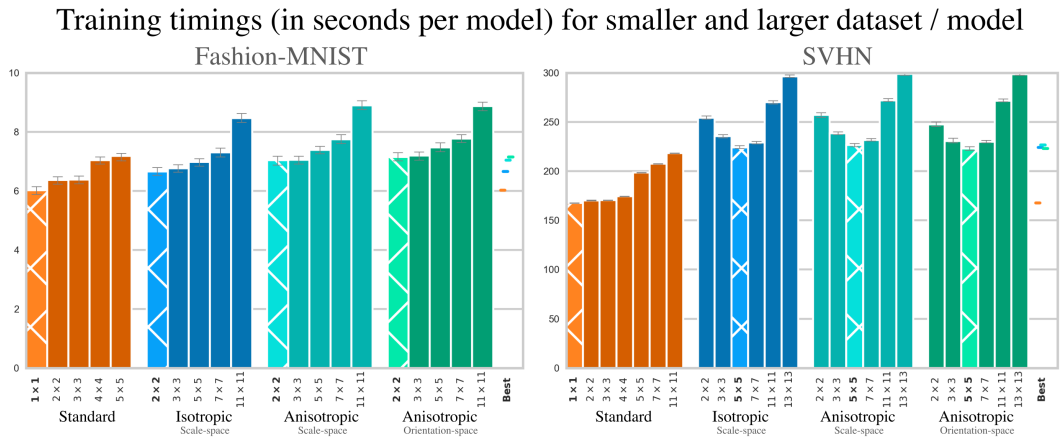
Figure 4.4: Seconds per model trained for Fashion-MNIST and SVHN datasets
