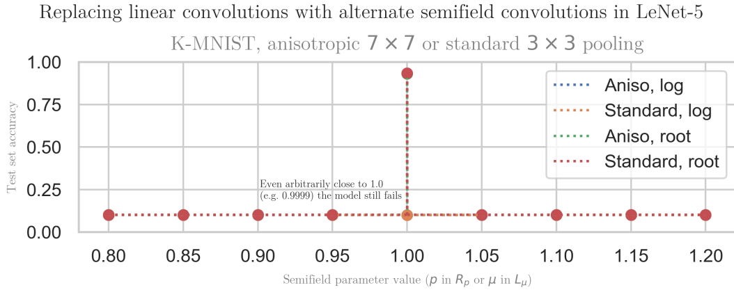
Figure 6.2: Results of nonlinear convolutions R_p and L_\mu for various p and \mu around 1. The pooling type does not seem to have a large effect (lines overlap).
