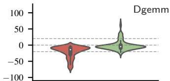
testbed-I
