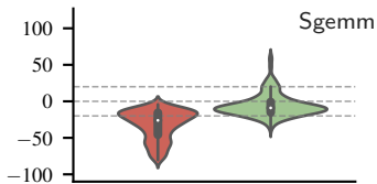
Prediction Error (%)
