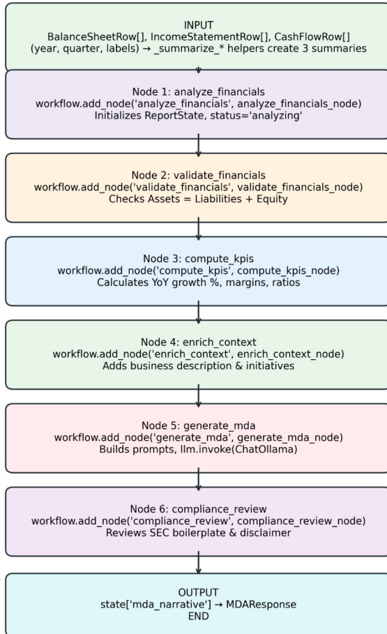
mda_agent.py - 6-Node LangGraph Workflow
