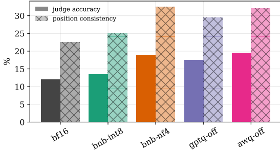
(a) EXT-2 JudgeBench
