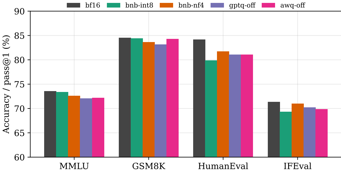
Quality by benchmark and quantization variant
