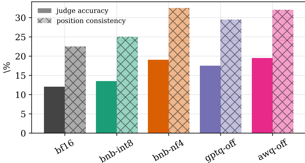
EXT-2 JudgeBench: pairwise judge accuracy \& position consistency
