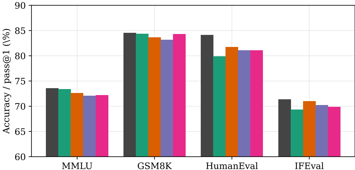
Quality by benchmark and quantization variant
