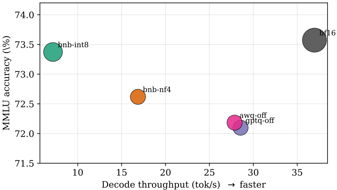
Quality-speed-memory trade-off (marker area \propto generate VRAM)
