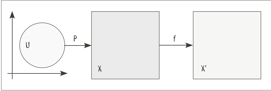
FIGURE 1.1. A smooth map f \in \mathcal{C}^\infty(X, X') .
